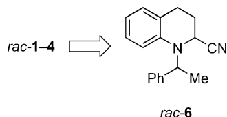
Scheme 1. Retrosynthesis of tetrahydroquinolines 1–4 .
