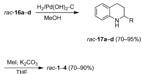
Scheme 6. Synthesis of tetrahydroquinoline alkaloids 1–4 .
