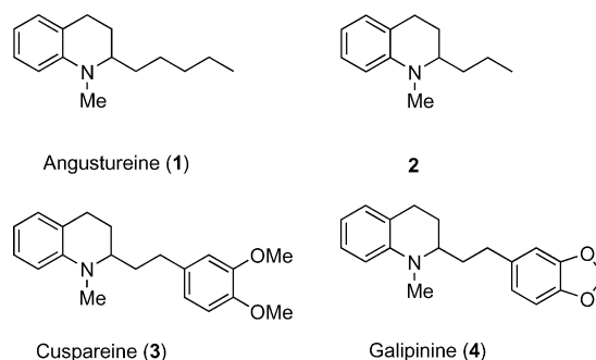
Figure 1. Structures of 2-substituted tetrahydroquinolines isolated from Galipea officinalis .
