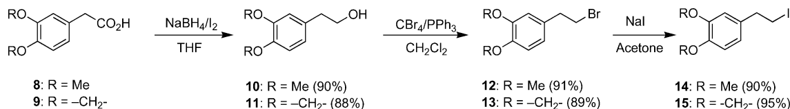
Scheme 4. Synthesis of alkyl halides 12–15 .
