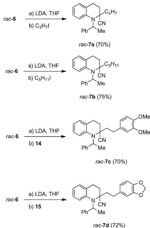
Scheme 3. Synthesis of \alpha -amino nitriles 7a–d .
