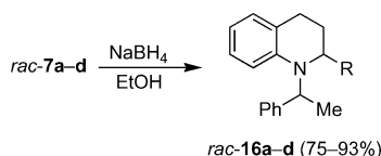
Scheme 5. Reductive decyanation of \alpha -amino nitriles 7a–d .
