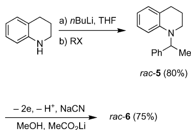
Scheme 2. Synthesis of \alpha -amino nitrile 6 .
