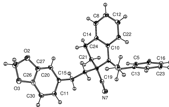
Figure 3. ORTEP drawing of \alpha -amino nitrile ( R^* , S^* )- 7d (for details see Table 5).
