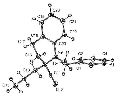
Figure 2. ORTEP drawing of \alpha -amino nitrile ( R^* , S^* )- 7a (for details see Table 5).
